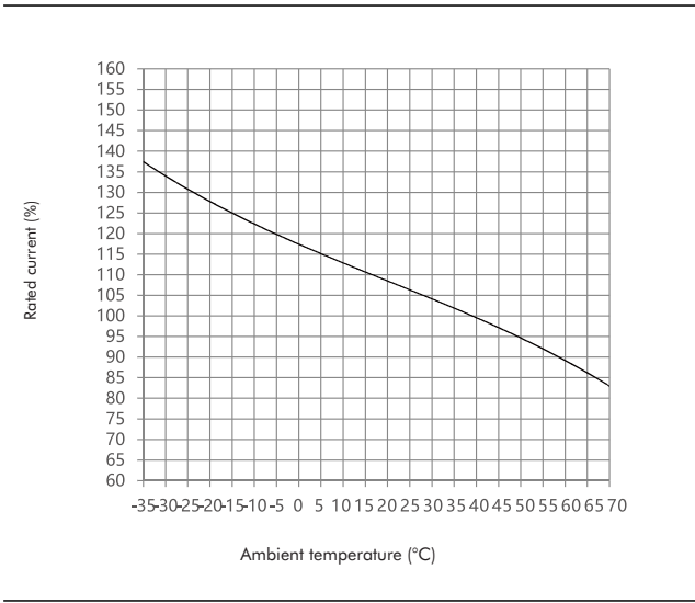
Temperature compensation curve
