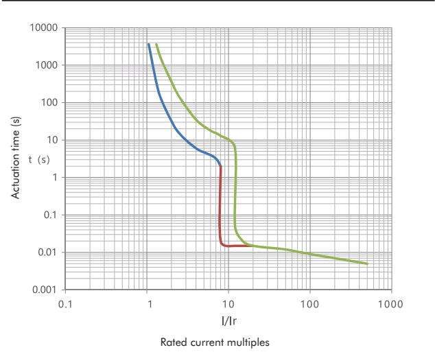
Tripping curve
