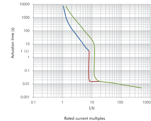
Tripping curve
