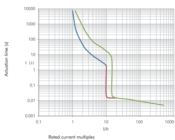
Tripping characteristic curve of motor protection
