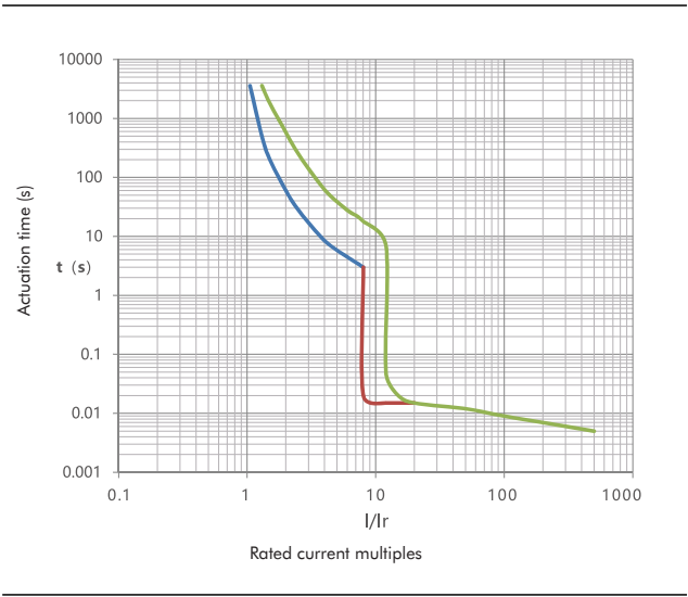
Tripping curve
