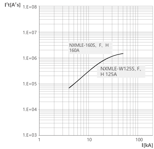
NXMLE-160(W125) Acceptable curves
