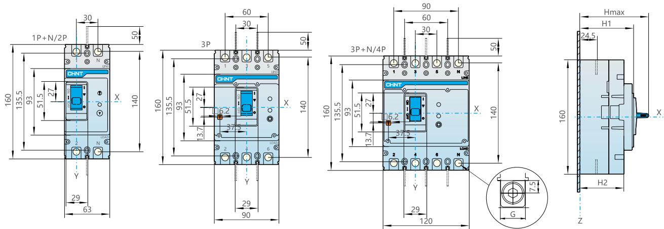
Front connection, dimension (mm)
