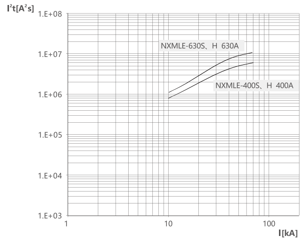
NXMLE-400/600 Acceptable curves
