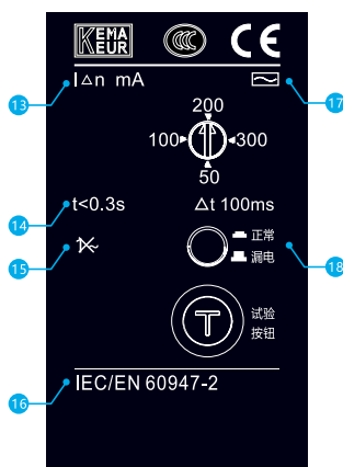
Nameplate of NXMLE residual current circuit breaker
